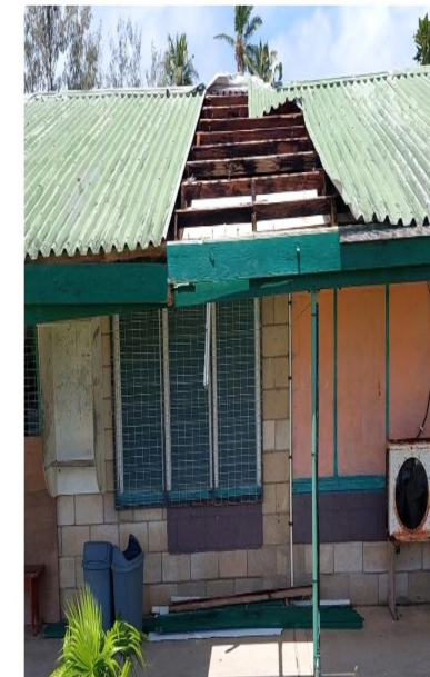
Onesua College - Roof Damage on Computer Lab
